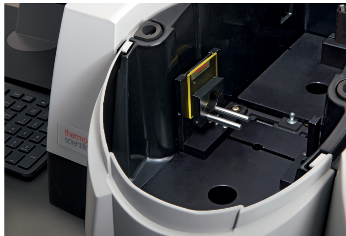
The Solid Sample Slide Holder positions accessories supplied on standard 2 x 3 inch slides. Instrument shown with a Universal Sample Holder and optional second slide holder.
